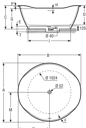
BAÑERA BETA ESSENTIAL V5 Ø140 / BETA ESSENTIAL V5 Ø140 BATHTUB / BAIGNOIRE BETA ESSENTIAL V5 Ø140 / BANHEIRA BETA ESSENTIAL V5 Ø140
