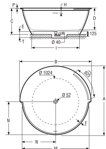
BAÑERA BETA ESSENTIAL V5 Ø140 / BETA ESSENTIAL V5 Ø140 BATHTUB / BAIGNOIRE BETA ESSENTIAL V5 Ø140 / BANHEIRA BETA ESSENTIAL V5 Ø140
