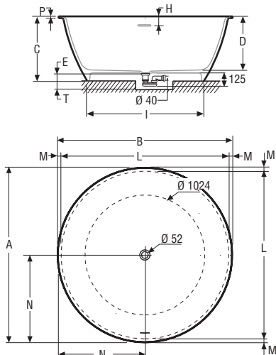
BAÑERA BETA ESSENTIAL V4 Ø127 / BETA ESSENTIAL V4 Ø127 BATHTUB / BAIGNOIRE BETA ESSENTIAL V4 Ø127 / BANHEIRA BETA ESSENTIAL V4 Ø127
