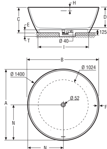
BAÑERA BETA ESSENTIAL V4 Ø140 / BETA ESSENTIAL V4 Ø140 BATHTUB / BAIGNOIRE BETA ESSENTIAL V4 Ø140 / BANHEIRA BETA ESSENTIAL V4 Ø140
