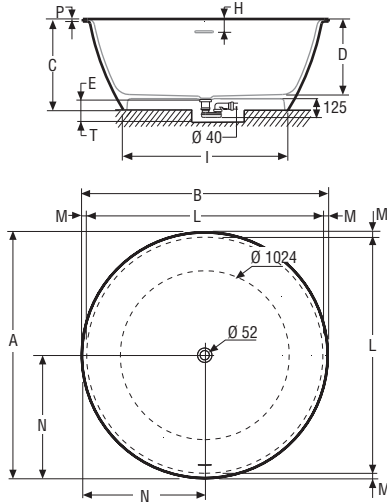
BAÑERA BETA ESSENTIAL V4 Ø140 / BETA ESSENTIAL V4 Ø140 BATHTUB / BAIGNOIRE BETA ESSENTIAL V4 Ø140 / BANHEIRA BETA ESSENTIAL V4 Ø140
