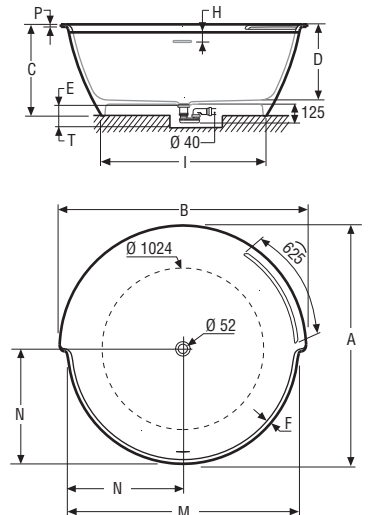
BAÑERA BETA ESSENTIAL V5 Ø150 / BETA ESSENTIAL V5 Ø150 BATHTUB / BAIGNOIRE BETA ESSENTIAL V5 Ø150 / BANHEIRA BETA ESSENTIAL V5 Ø150
